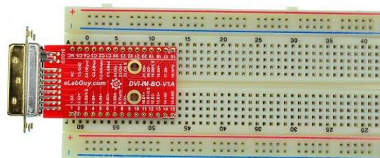
Figure 2: Example of connecting the DVI-IM-BO-V1A on a breadboard
