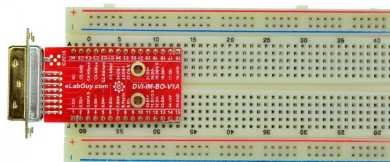
Figure 2: Example of connecting the DVI-DM-BO-V1A on a breadboard
