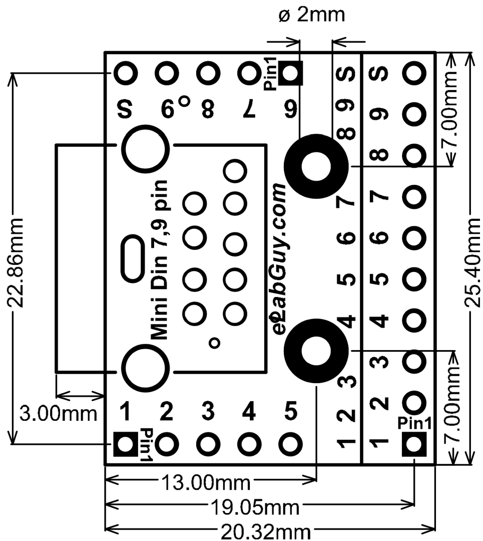
mDin-F-BO-V2A PCB outline Drawing
