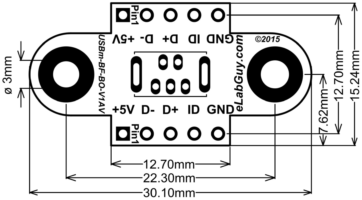
USBm-BF-BO-V1AV Schematic Diagram
