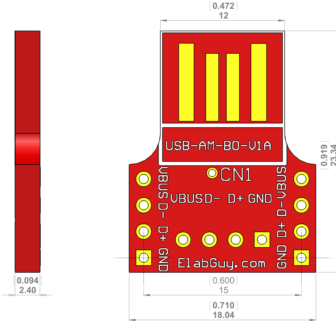
USB-AM-BO-V1A PCB Outline Drawing
