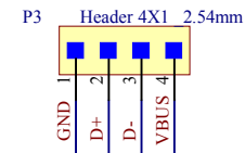
USB-AM-BO-V1A Schematic Diagram
