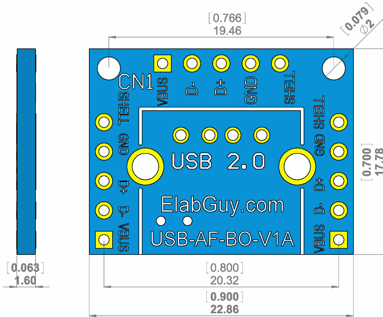
USB-AF-BO-V1A PCB Outline Drawing
