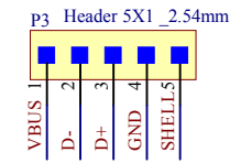
USB-AF-BO-V1A Schematic Diagram
