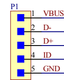
Header 5X1 _2.54mm
