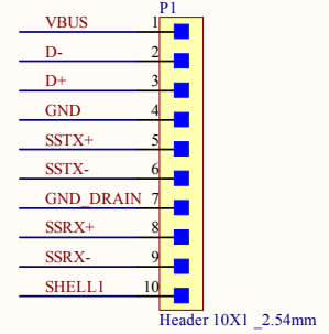
USB3-AM-BO-V1A Schematic Diagram
