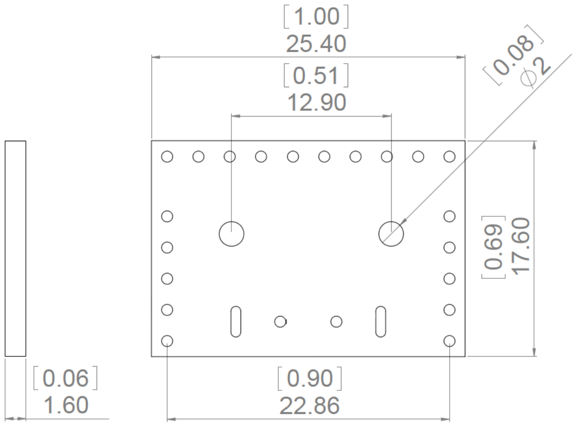
USB3-AM-BO-V1A PCB Outline Drawing
