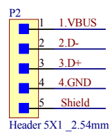
Header 5X1 2.54mm
