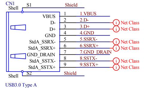
USB3.0 Type A
