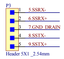
Header 5X1 2.54mm
