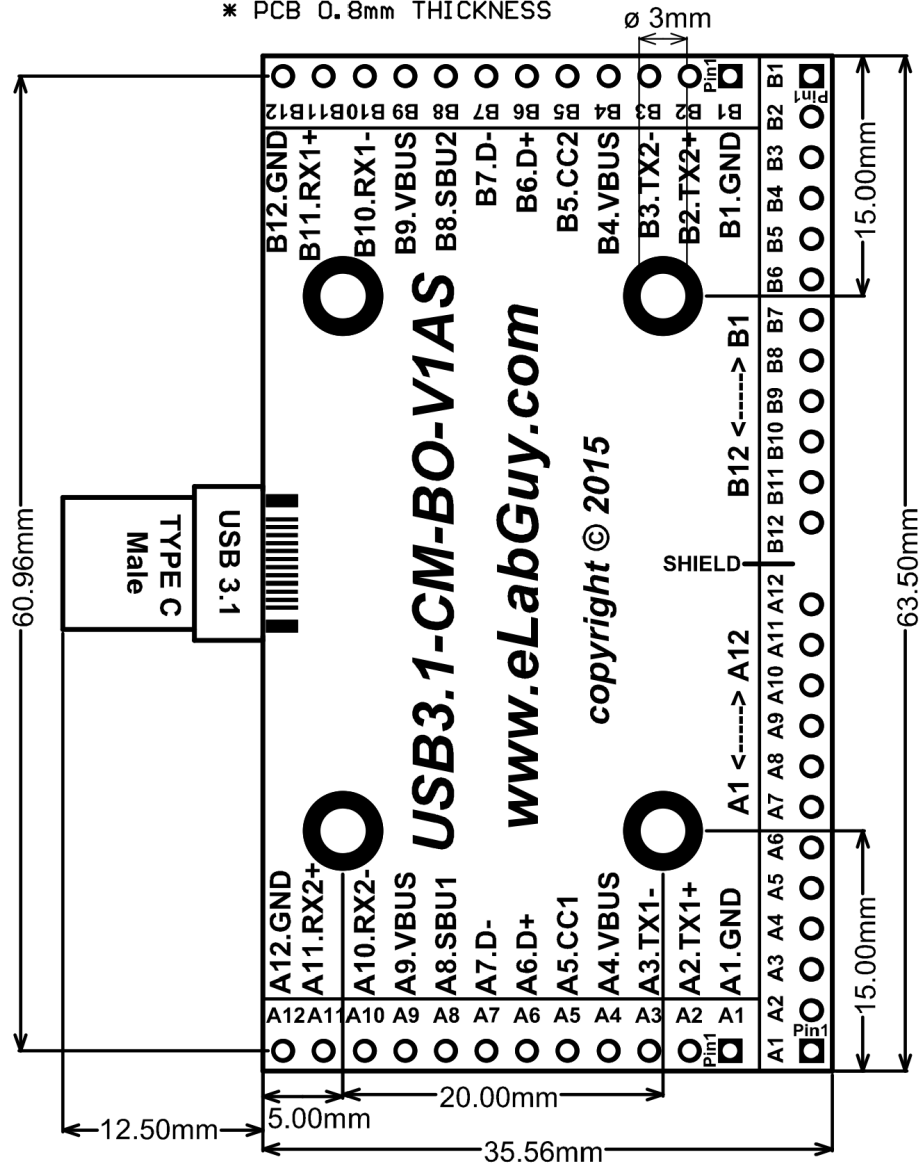
USB3.1-CM-BO-V1AS PCB outline Drawing
