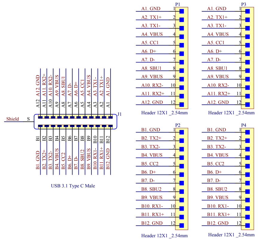
USB3.1-CM-BO-V1AS Schematic Diagram
