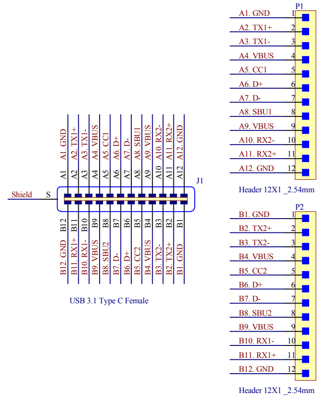
USB3.1-CF-BO-V2A Schematic Diagram
