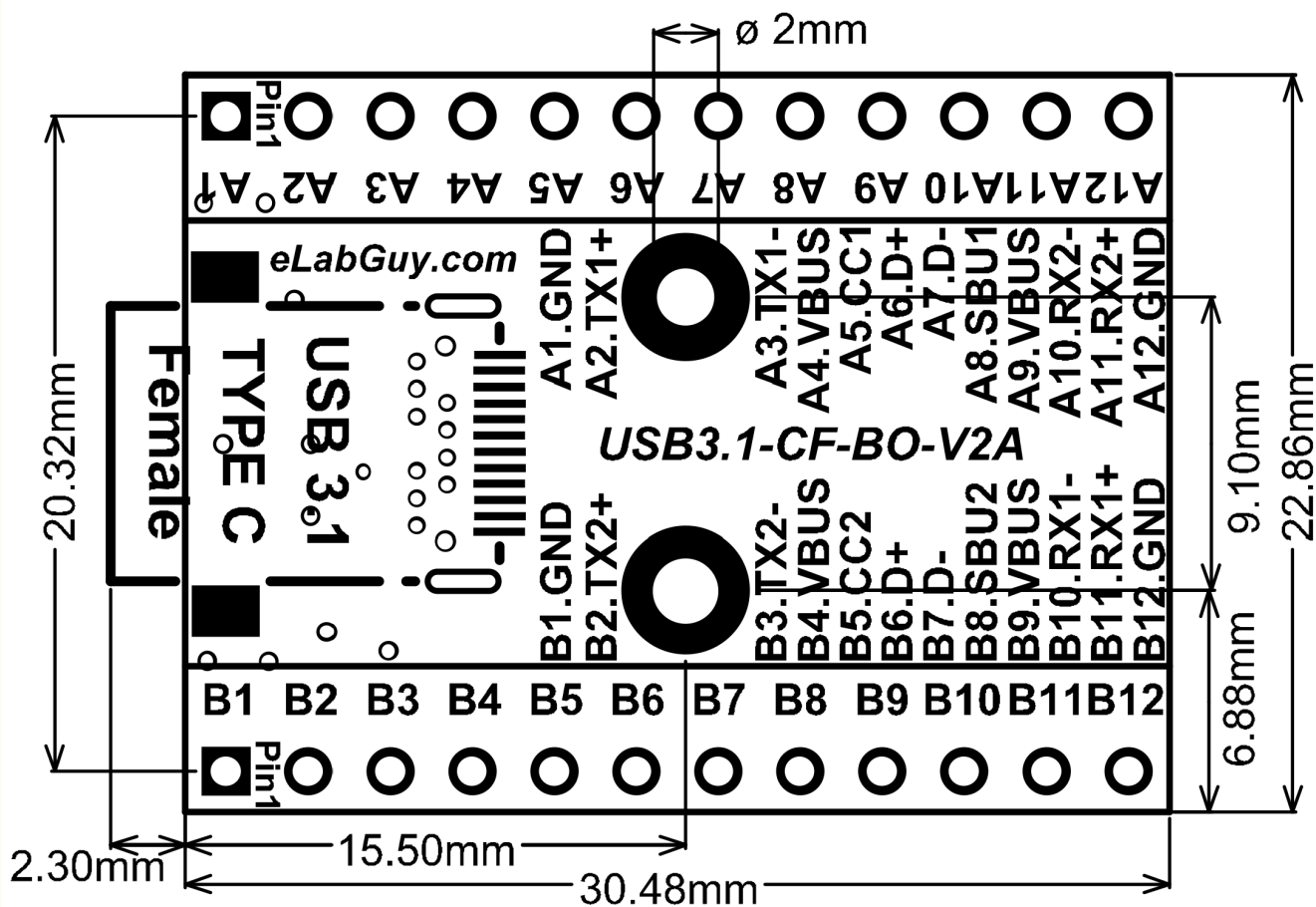
PCB outline Drawing
