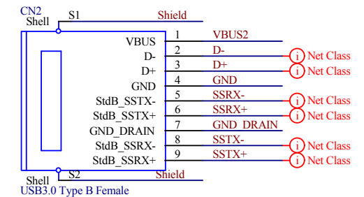
USB3.0 Type B Female
