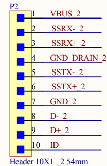
Header 10X1_2.54mm
