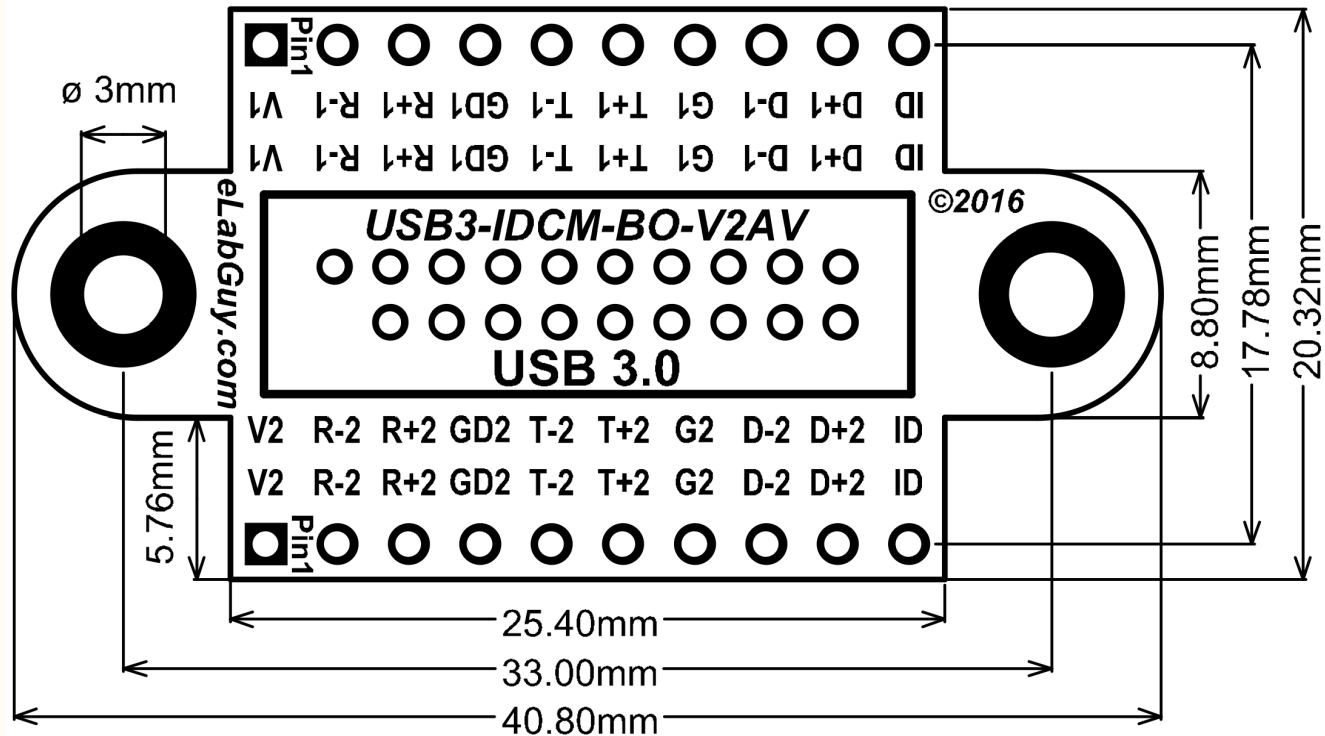
PCB outline Drawing
