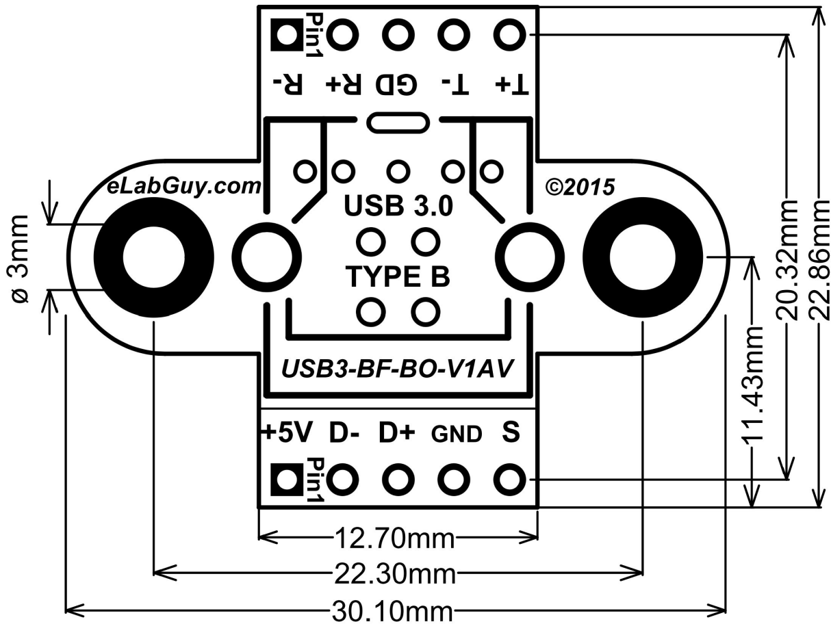
USB3-BF-BO-V1AV PCB outline Drawing
