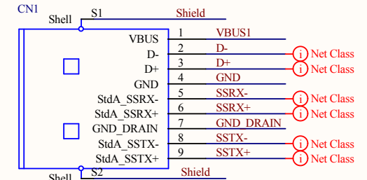
USB3.0 Type A male plug
