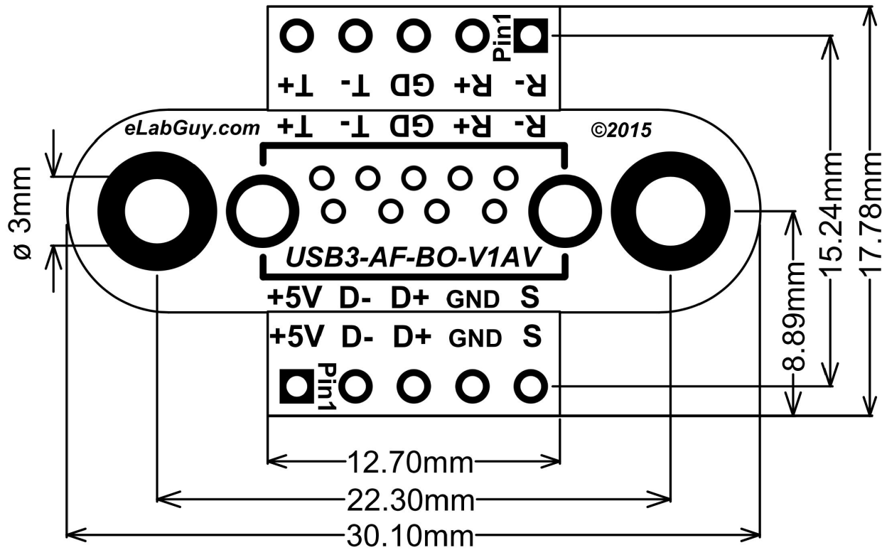
USB3-AF-BO-V1AV Schematic Diagram
