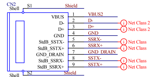
USB3.0 Type B Female
