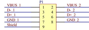
Header 5X1_4X1_2.54mm_USB_DUAL
