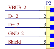
Header 5X1_2.54mm
