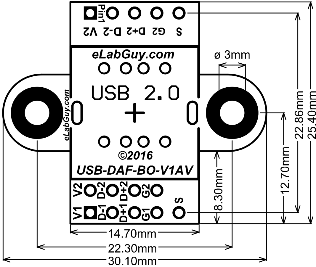
USB-DAF-BO-V1AV PCB outline Drawing
