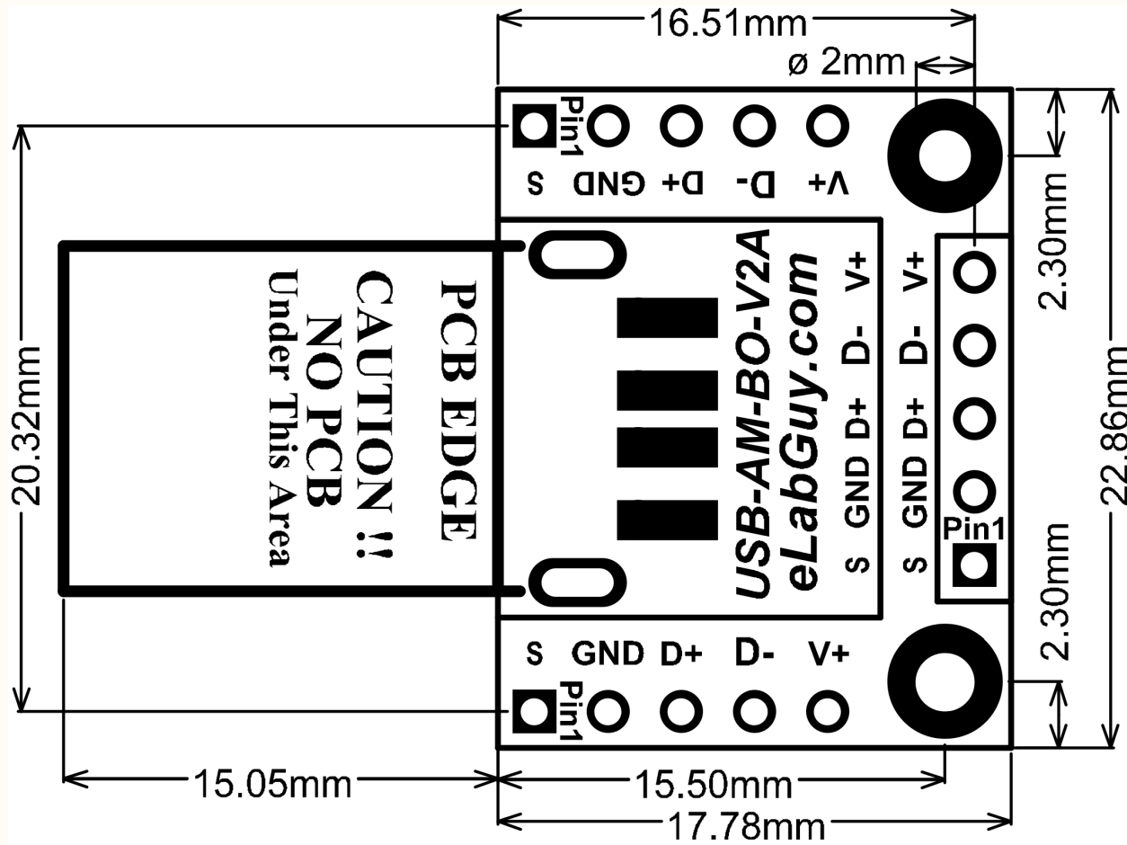
PCB outline Drawing
