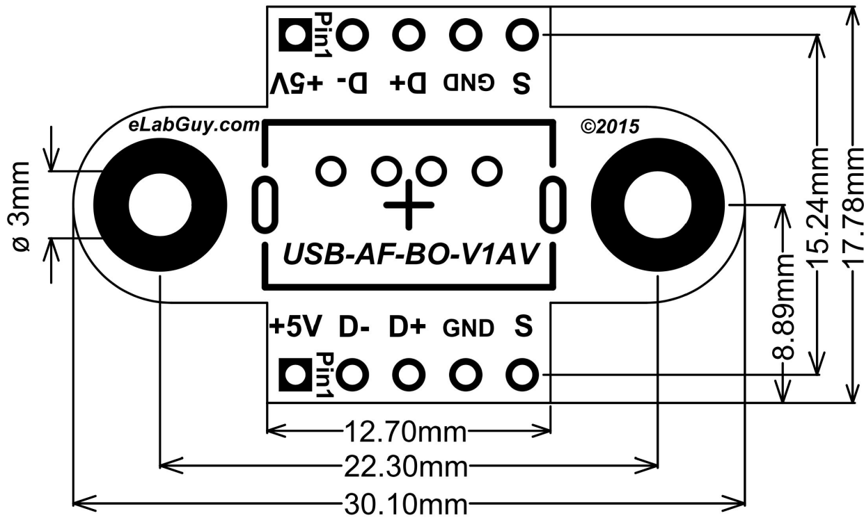
USB-AF-BO-V1AV PCB outline Drawing
