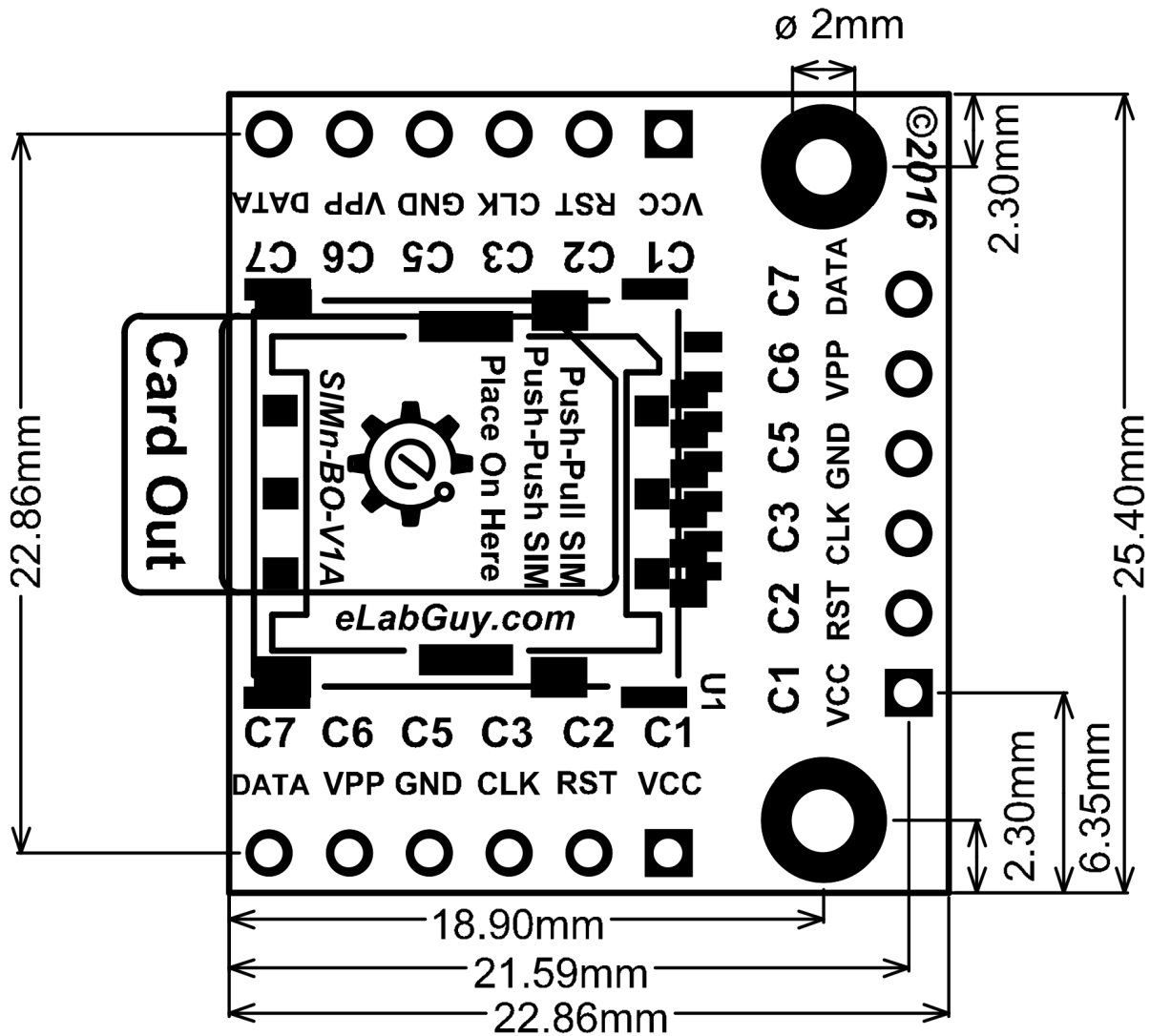
PCB outline Drawing
