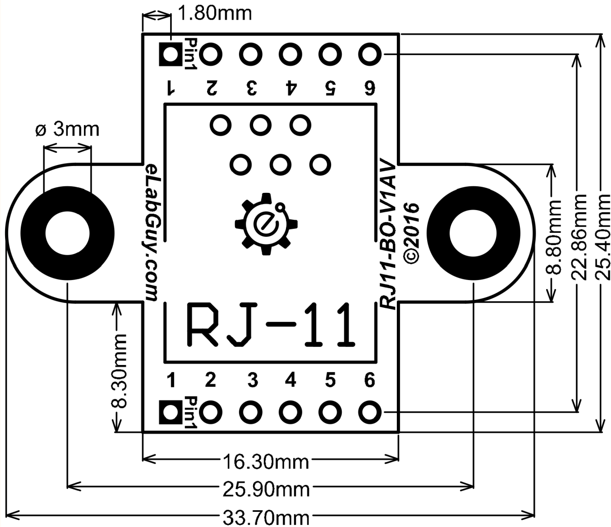
PCB outline Drawing
