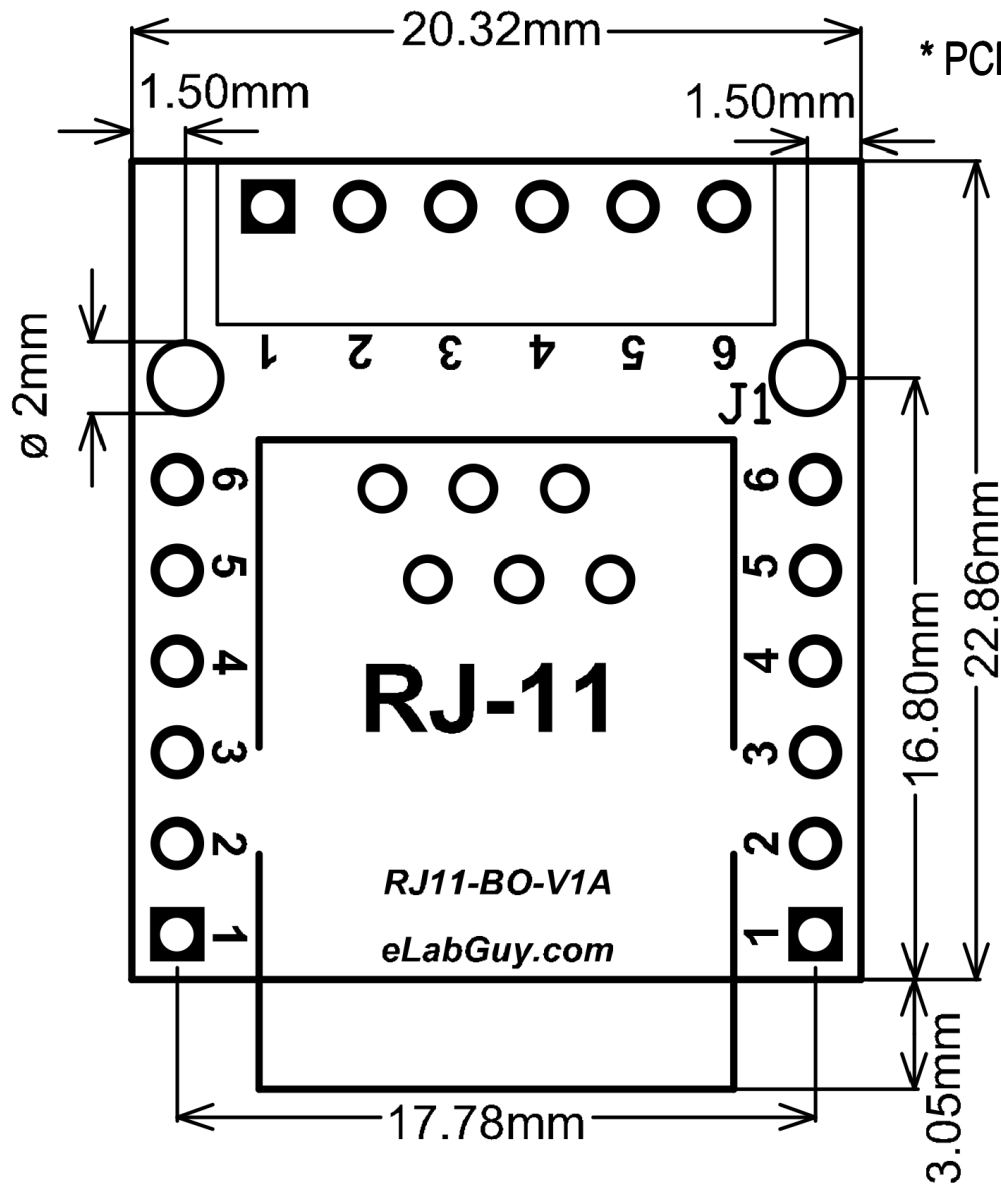
RJ11-BO-V1A PCB outline Drawing
