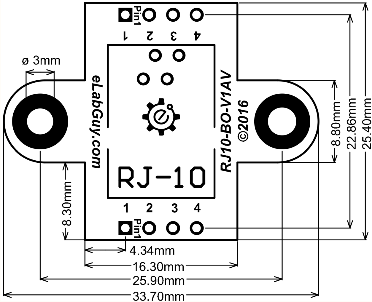
PCB outline Drawing
