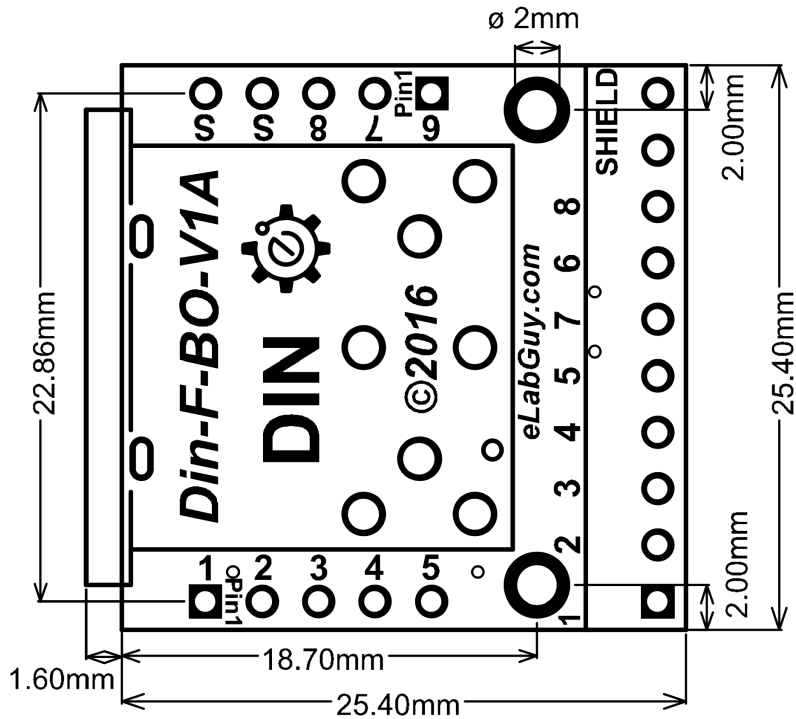
Din-F-BO-V1A PCB outline Drawing
