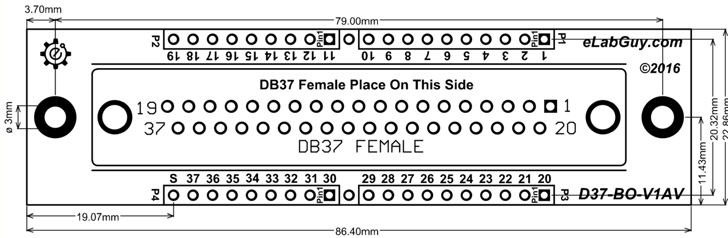
PCB outline Drawing
