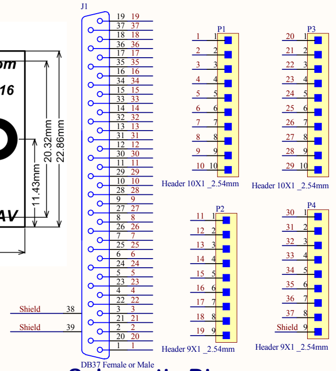
DB37 Female or Male Schematic Diagram
