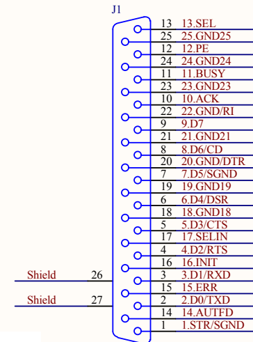
DB25 Female or Male
