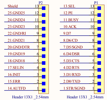
Schematic Diagram
