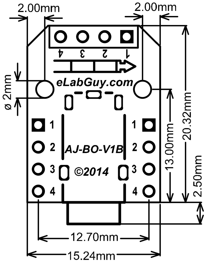
AJ-BO-V1B PCB outline Drawing
