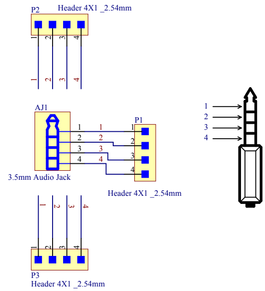
AJ-BO-V1B Schematic Diagram
