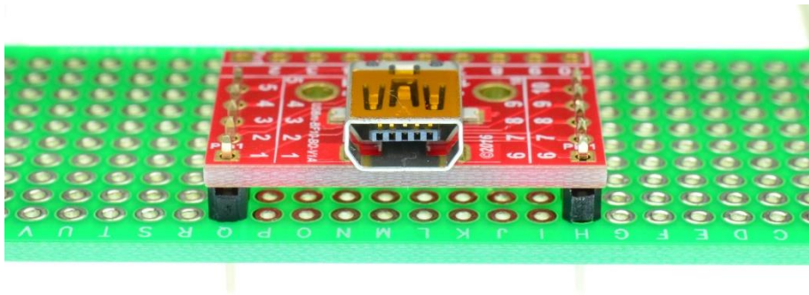
Figure 5: Solid Mounting on prototype PCB
