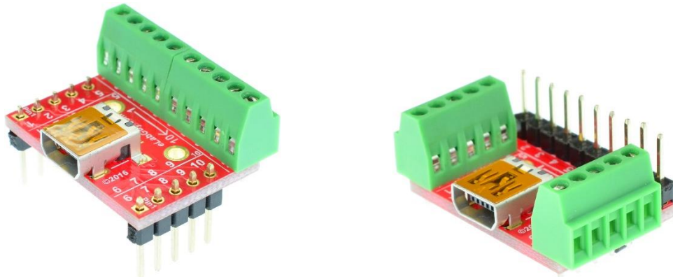
Figure 3: USBm-BF10-BO-V1A Various connections
