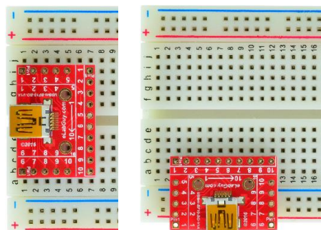
Figure 2: Example of connecting the USBm-BF10-BO-V1A on a breadboard
