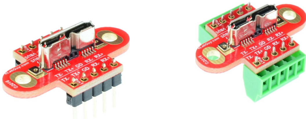
Figure 3: USB3u-BF-BO-V1AV Various connections
