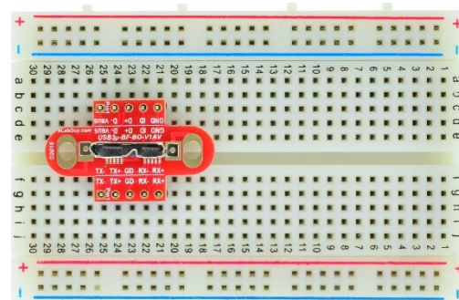
Figure 2: Example of connecting the USB3u-BF-BO-V1AV on a breadboard
