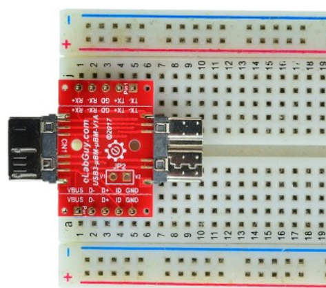
Figure 2: Example of connecting the USB3-uBM-uBM-V1A on a breadboard (Note: This picture only shows the pins spacing, actual use may not be used on a breadboard)
