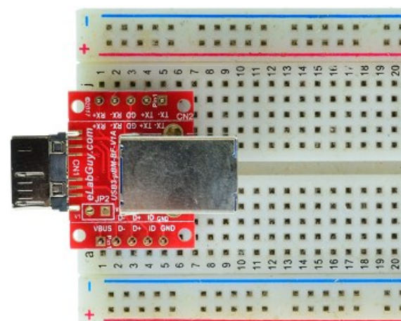
Figure 2: Example of connecting the USB3-uBM-BF-V1A on a breadboard (Note: This picture only shows the pins spacing, actual use may not be used on a breadboard)
