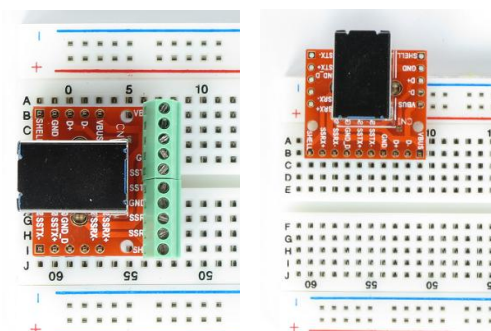
Figure 2: Examples of various methods for connecting the USB3-BF-BO-V1A to a breadboard
