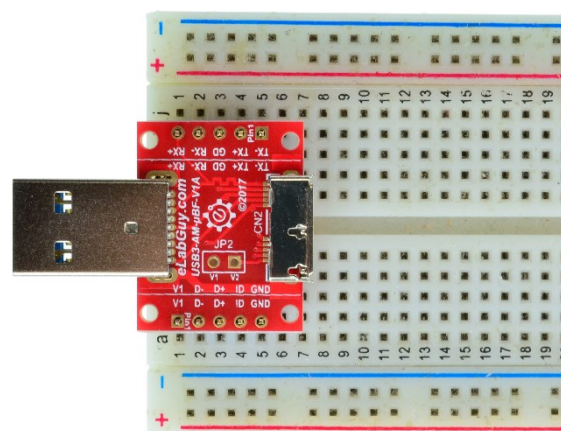
Figure 2: Example of connecting the USB3-AM-uBF-V1A on a breadboard (Note: This picture only shows the pins spacing, actual use may not be used on a breadboard)
