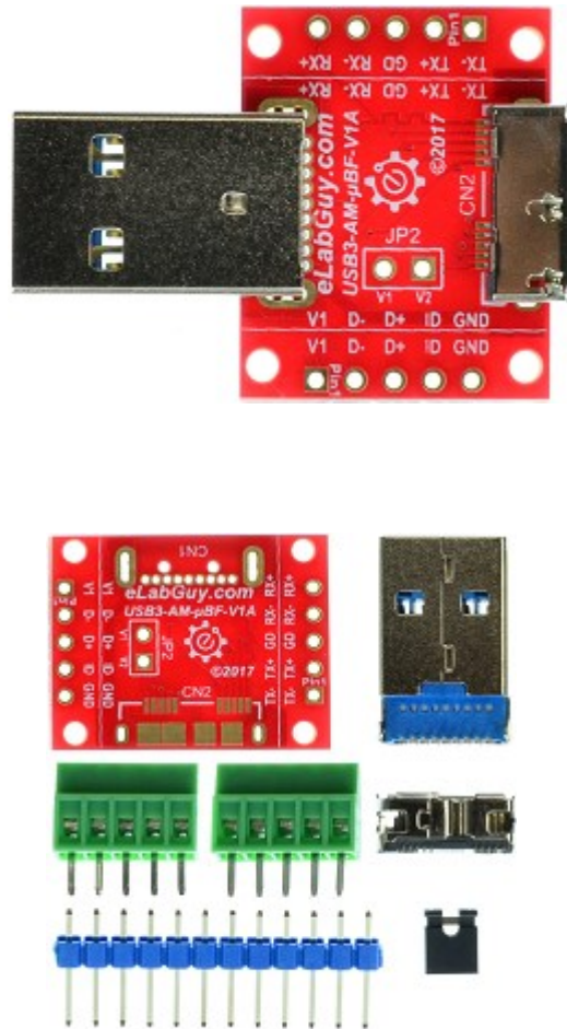
Figure 1: Parts inside the kit (Note: the module is not assembled, user can decide which connector to use on the module.)
