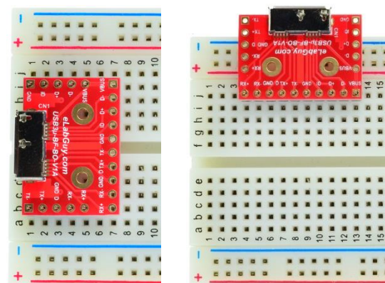
Figure 2: Example of connecting the USB3 \mu -BF-BO-V1A on a breadboard
