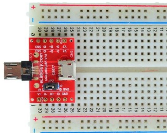
Figure 2: Example of connecting the USB-uBM-uBF-V1A on a breadboard (Note: This picture only shows the pins spacing, actual use may not be used on a breadboard)
