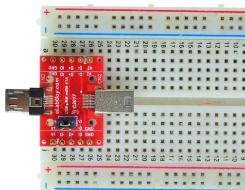
Figure 2: Example of connecting the USB-uBM-mBM-V1A on a breadboard (Note: This picture only shows the pins spacing, actual use may not be used on a breadboard)
