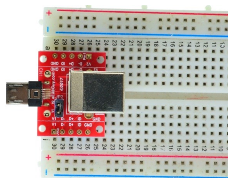
Figure 2: Example of connecting the USB-uBM-BF-V1A on a breadboard (Note: This picture only shows the pins spacing, actual use may not be used on a breadboard)
