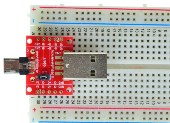
Figure 2: Example of connecting the USB-uBM-AM-V1A on a breadboard (Note: This picture only shows the pins spacing, actual use may not be used on a breadboard)
