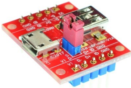
Figure 3: USB-uBF-mBF-V1A with headers
