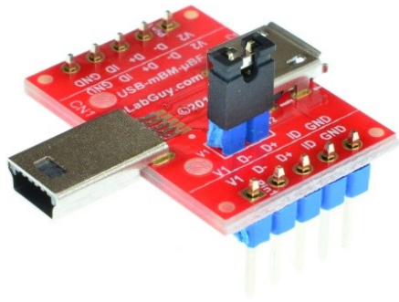
Figure 3: USB-mBM-uBF-V1A with headers
