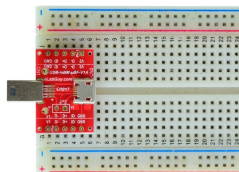
Figure 2: Example of connecting the USB-mBM-uBF-V1A on a breadboard (Note: This picture only shows the pins spacing, actual use may not be used on a breadboard)
