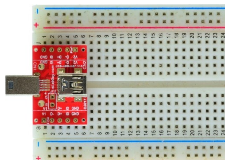
Figure 2: Example of connecting the USB-mBM-mBF-V1A on a breadboard (Note: This picture only shows the pins spacing, actual use may not be used on a breadboard)
