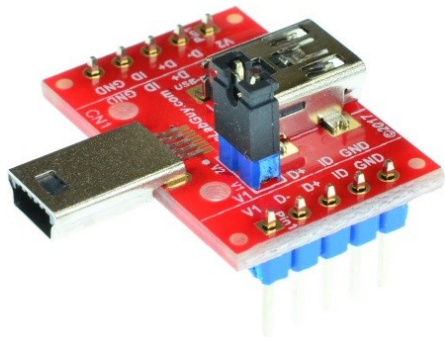
Figure 3: USB-mBM-mBF-V1A with headers
