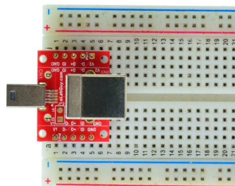
Figure 2: Example of connecting the USB-mBM-BF-V1A on a breadboard (Note: This picture only shows the pins spacing, actual use may not be used on a breadboard)
