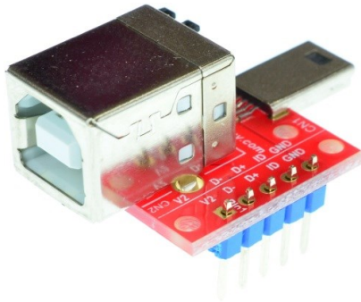
Figure 3: USB-mBM-BF-V1A with headers
