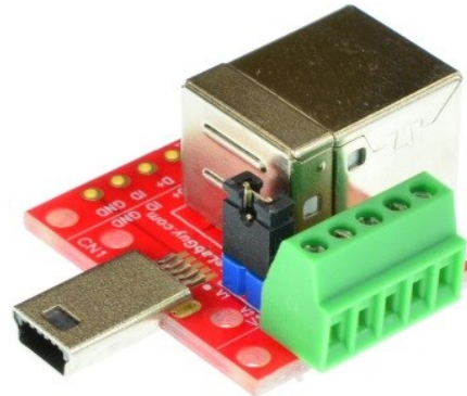
Figure 4: USB-mBM-BF-V1A with terminal blocks
