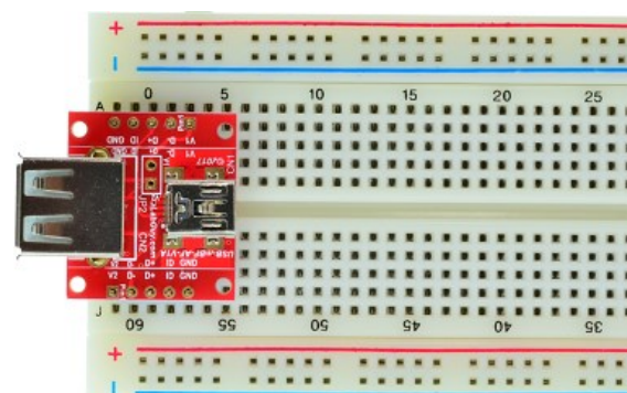
Figure 2: Example of connecting the USB-mBF-AF-V1A on a breadboard (Note: This picture only shows the pins spacing, actual use may not be used on a breadboard)
