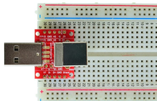
Figure 2: Example of connecting the USB-AM-BF-V1A on a breadboard (Note: This picture only shows the pins spacing, actual use may not be used on a breadboard)
