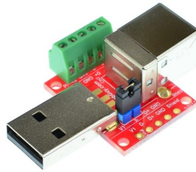
Figure 4: USB-AM-BF-V1A with terminal blocks
