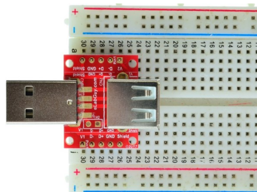
Figure 2: Example of connecting the USB-AM-AF-V1A on a breadboard (Note: This picture only shows the pins spacing, actual use may not be used on a breadboard)
