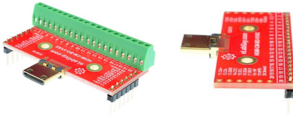
Figure 3: HDMI-CM-BO-V1AS Various connections
