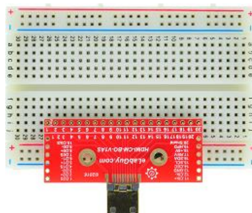
Figure 2: Example of connecting the HDMI-CM-BO-V1AS on a breadboard
