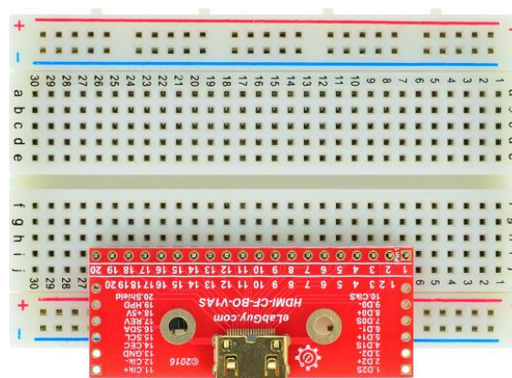
Figure 2: Example of connecting the HDMI-CF-BO-V1AS on a breadboard
