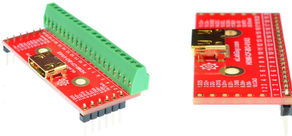
Figure 3: HDMI-CF-BO-V1AS Various connections
