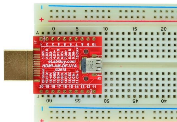
Figure 2: Example of connecting the HDMI-AM-DF-V1A on a proto PCB (Note: This picture only shows the pins spacing, actual use may not be used on a breadboard)
