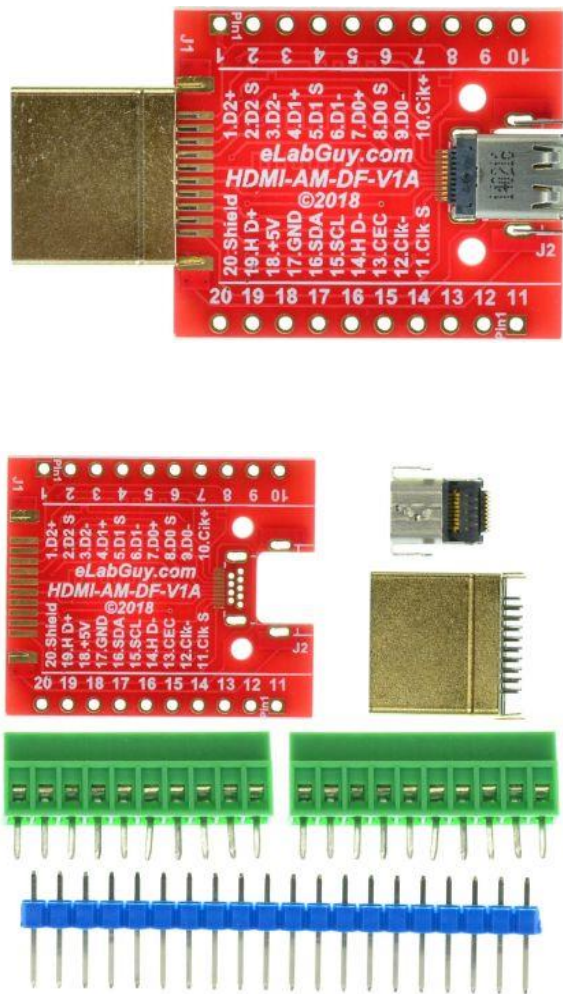
Figure 1: Parts inside the kit (Note: the module is not assembled, user can decide which connector to use on the module.)
