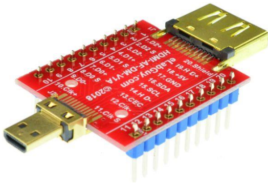
Figure 3: HDMI-AF-DM-V1A with headers
