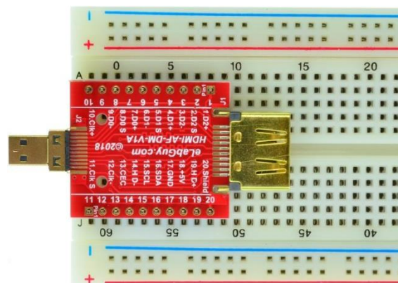
Figure 2: Example of connecting the HDMI-AF-DM-V1A on a proto PCB (Note: This picture only shows the pins spacing, actual use may not be used on a breadboard)
